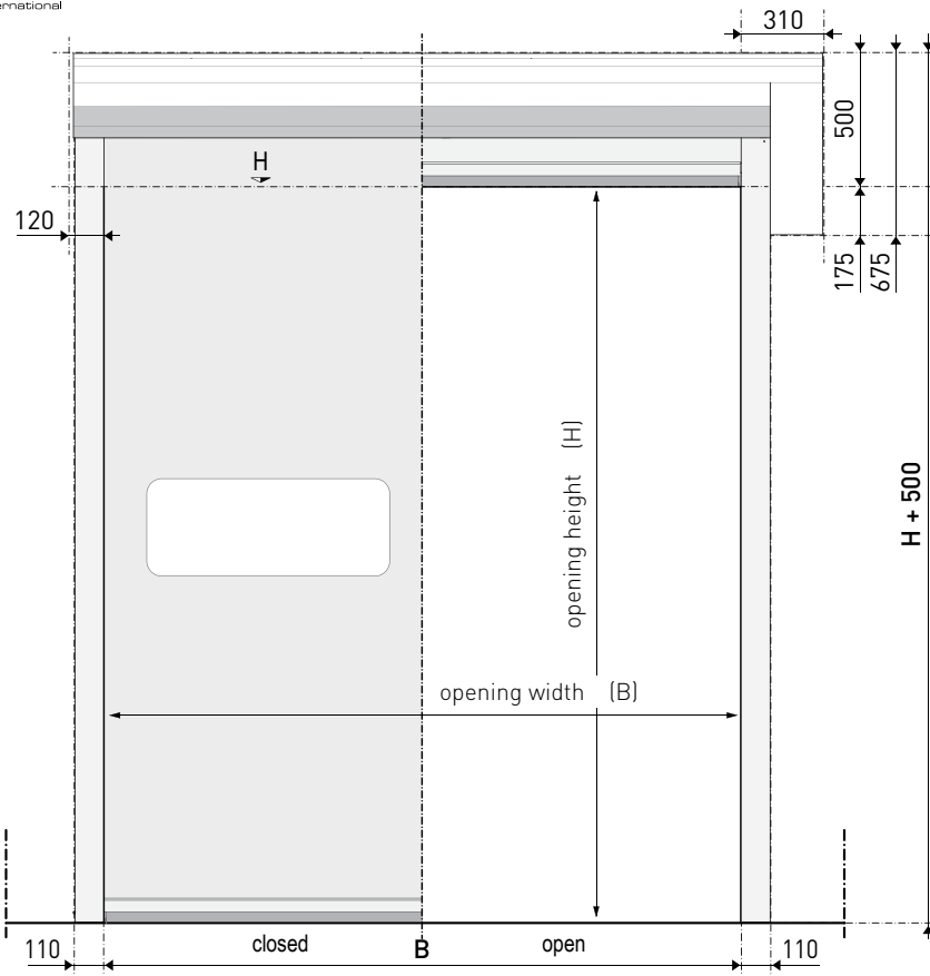
[ Front view ]
