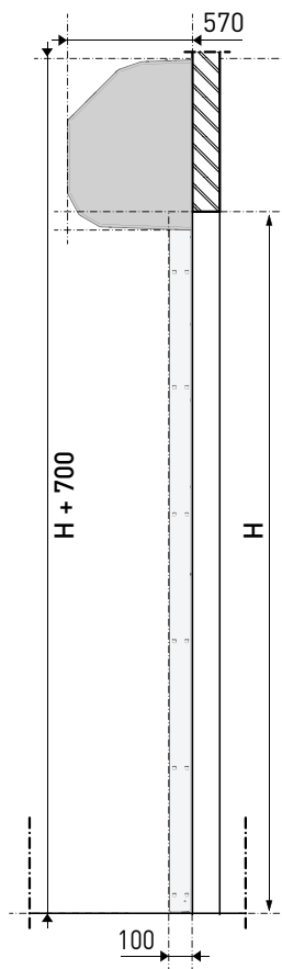
[ Coupe transversale ]
