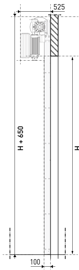
[ Coupe transversale ]
