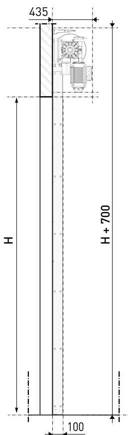
[ Coupe transversale ]
