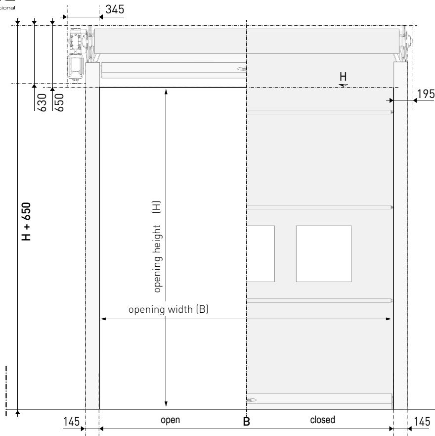
[ Drive side ]
