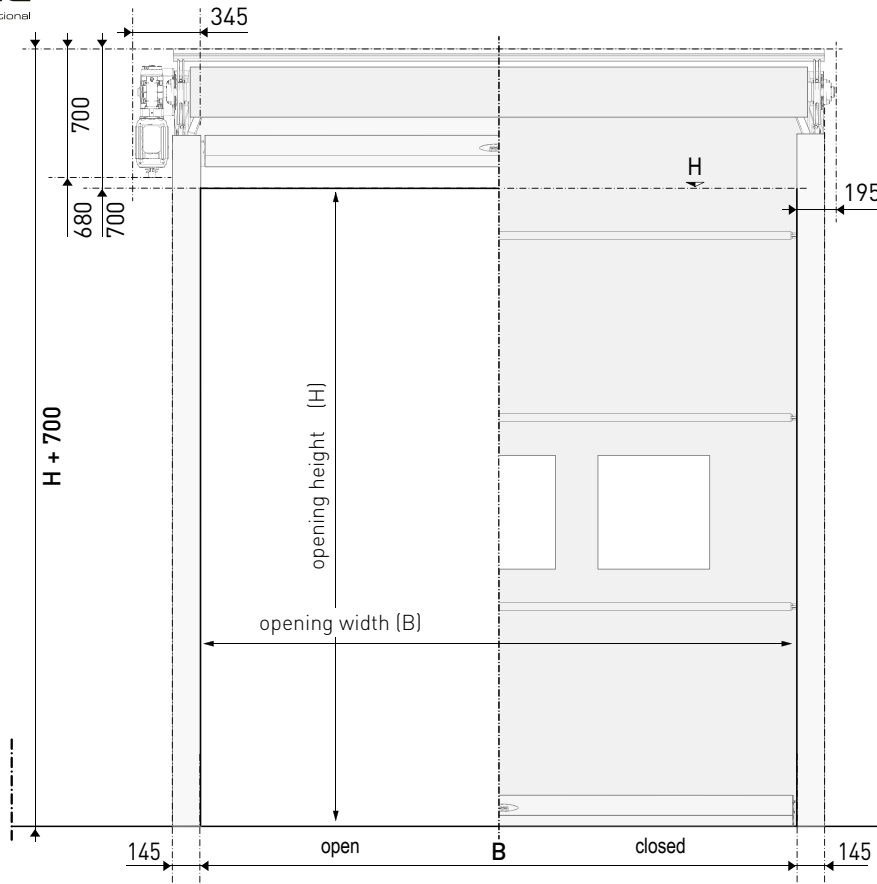
[ Drive side ]
