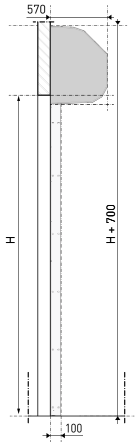
[ Cross section ]
