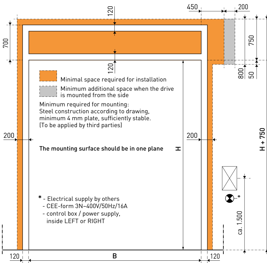
— [ Front view ]
