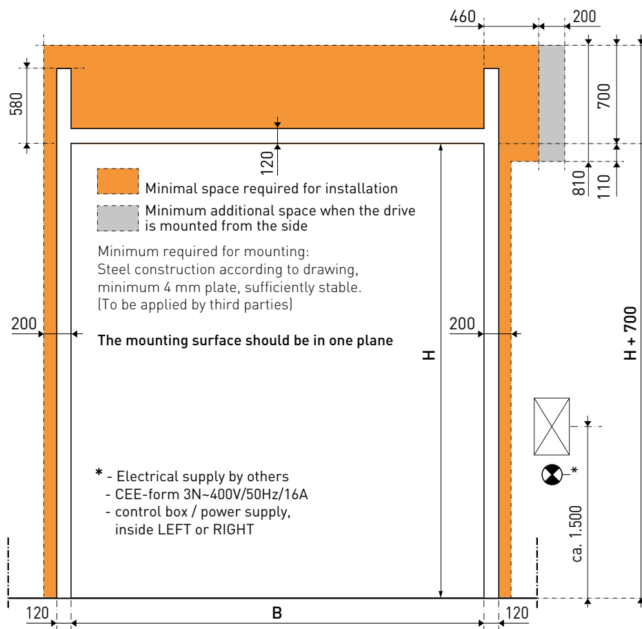
— [ Front view ]
