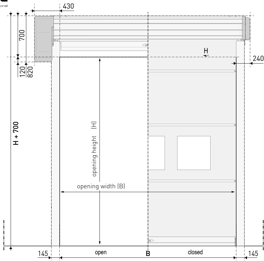
[ Drive side ]
