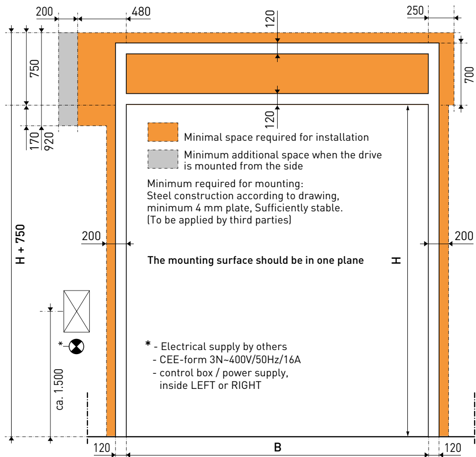
[ Drive side ]
