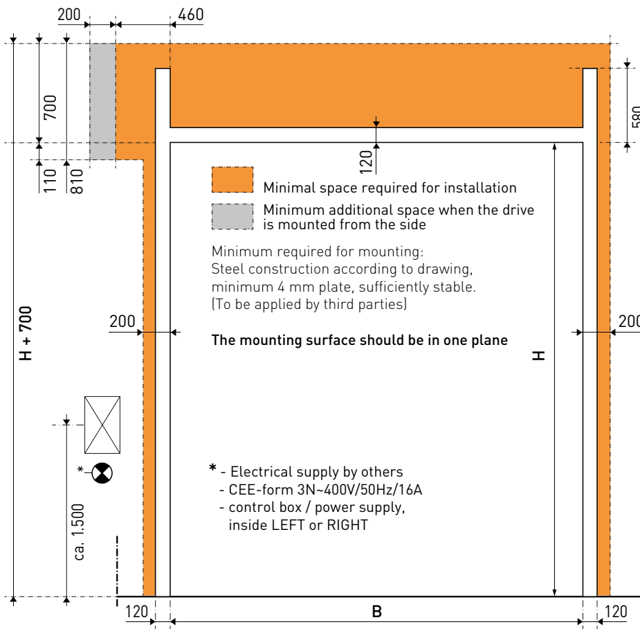
[ Drive side ]
