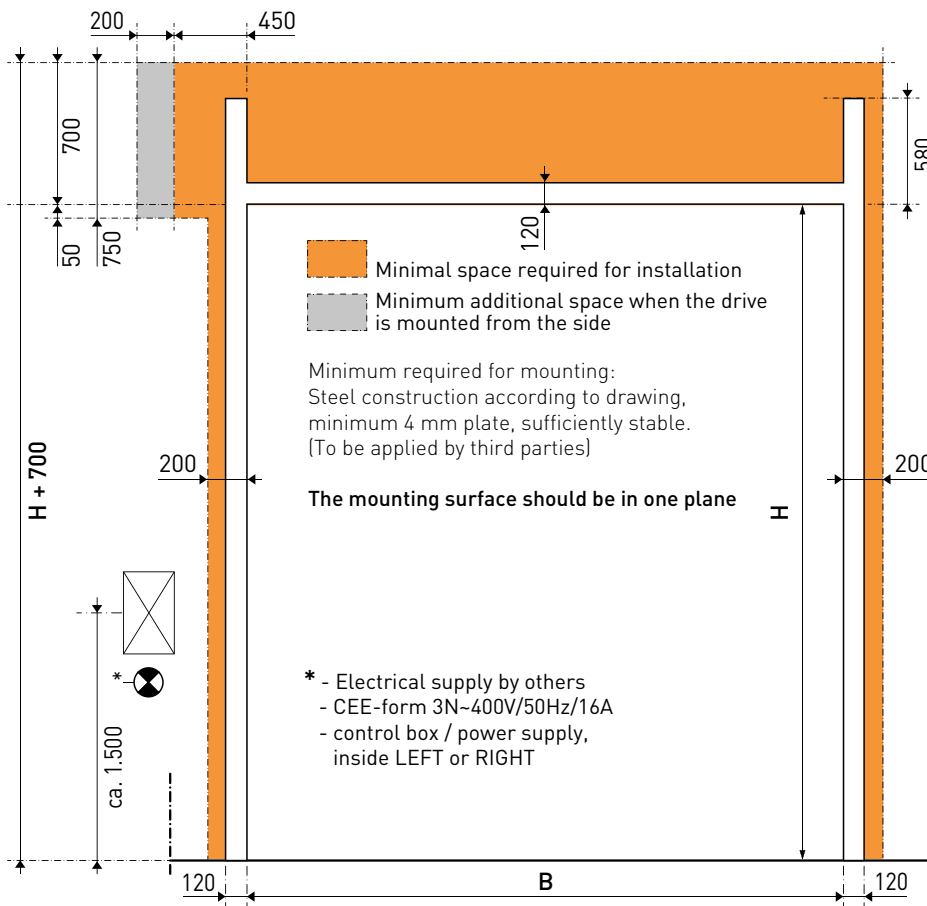
[ Drive side ]
