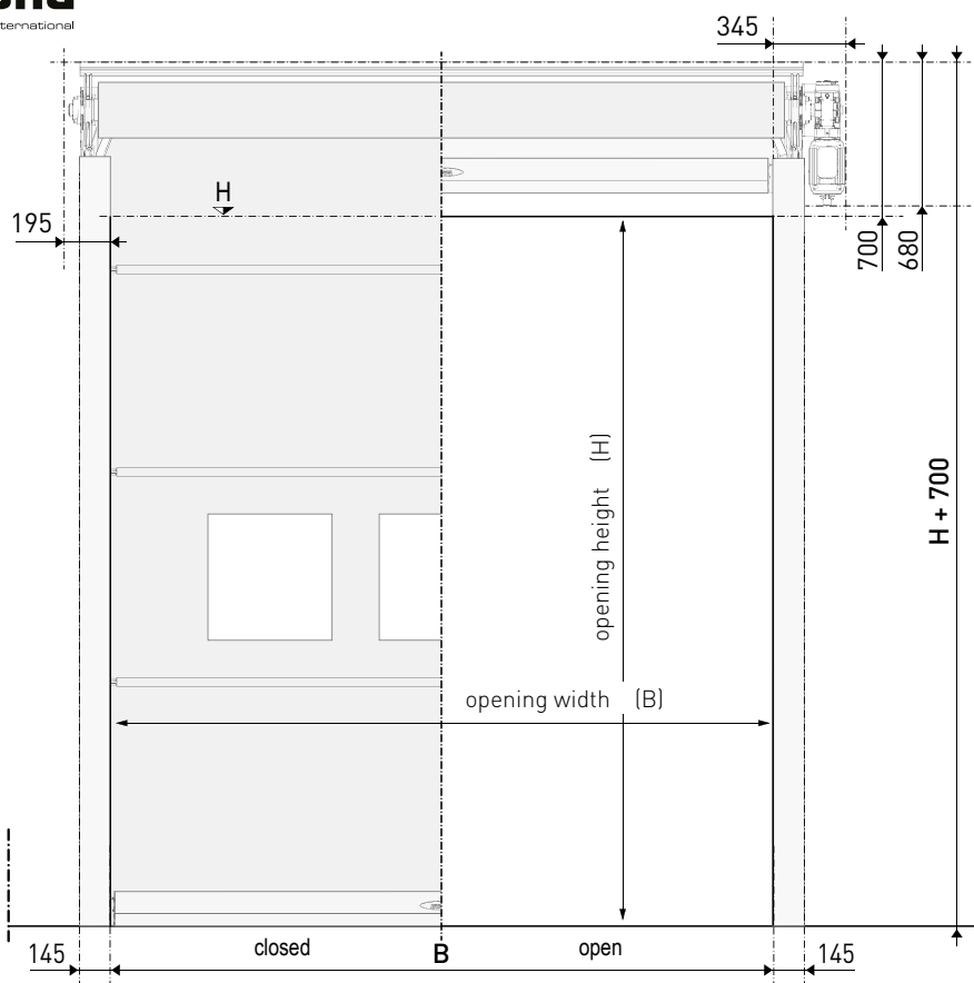
— [ Front view ]
