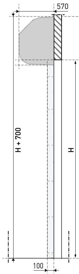
[ Cross section ]
