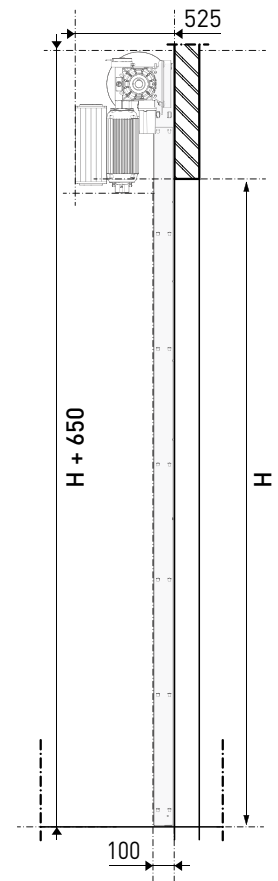
[ Cross section ]
