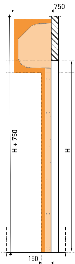
[ Cross section ]
