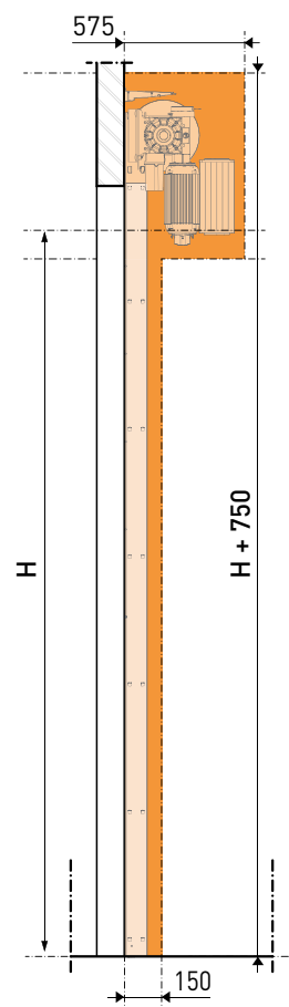
— [ Cross section ]
